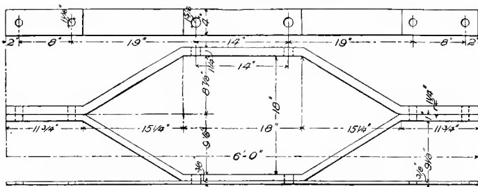
Figs. 4619-4652. Upper and Lower Arch-bars and Tie-bar (2 of each).
